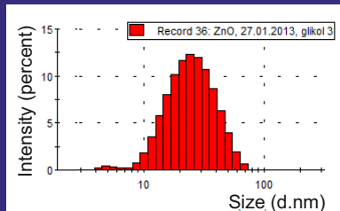
Histogram of the particle size distribution, DLS
